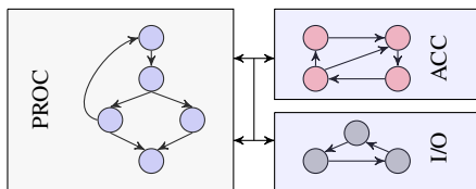
Fig. 2: Instruction-Level Abstraction
